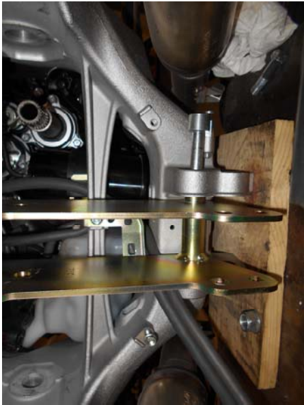
55 front chassis mounting bracket
